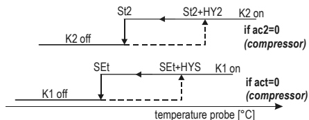
Fig. 2 - exemple of 2 independent stages SYS=1
