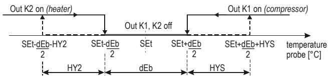
Fig. 3 - Dead band control SYS=2
